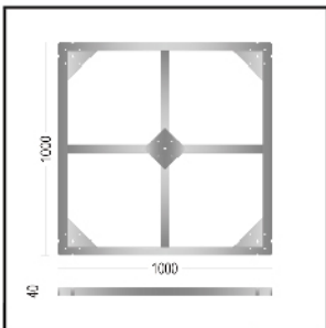
Aluminium frame
