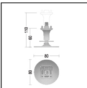
Adjustable foot. Zinc
